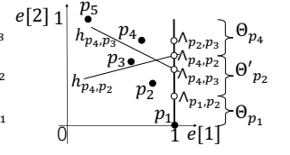
Figure 4: Division of S_4
